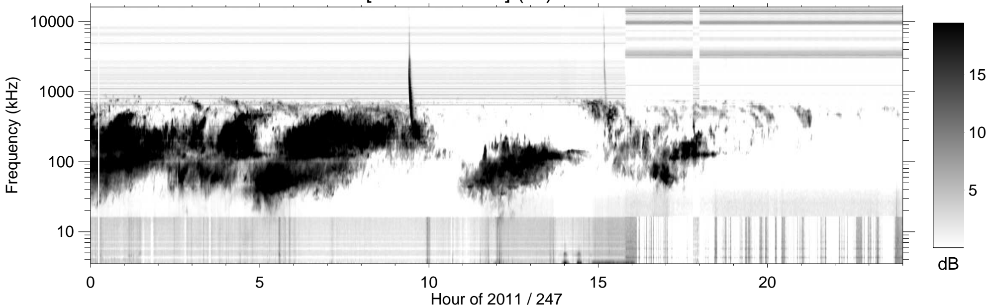
RPWS [ABCH1H2/Ex] (-B) 2011/09/04
