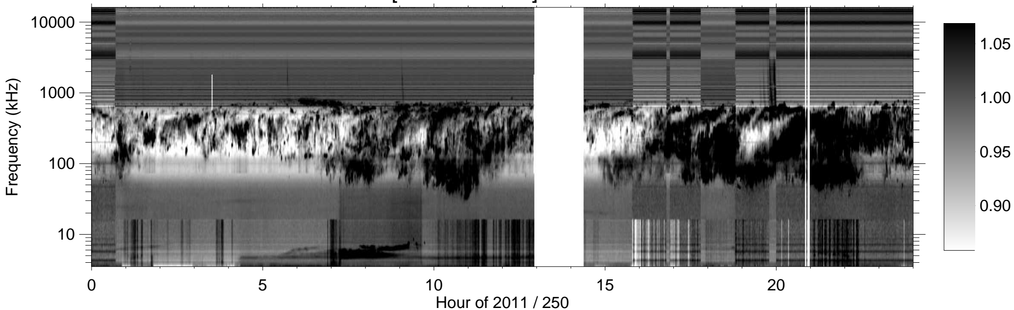
RPWS [ABCH1H2/Ex] (-B) 2011/09/07
