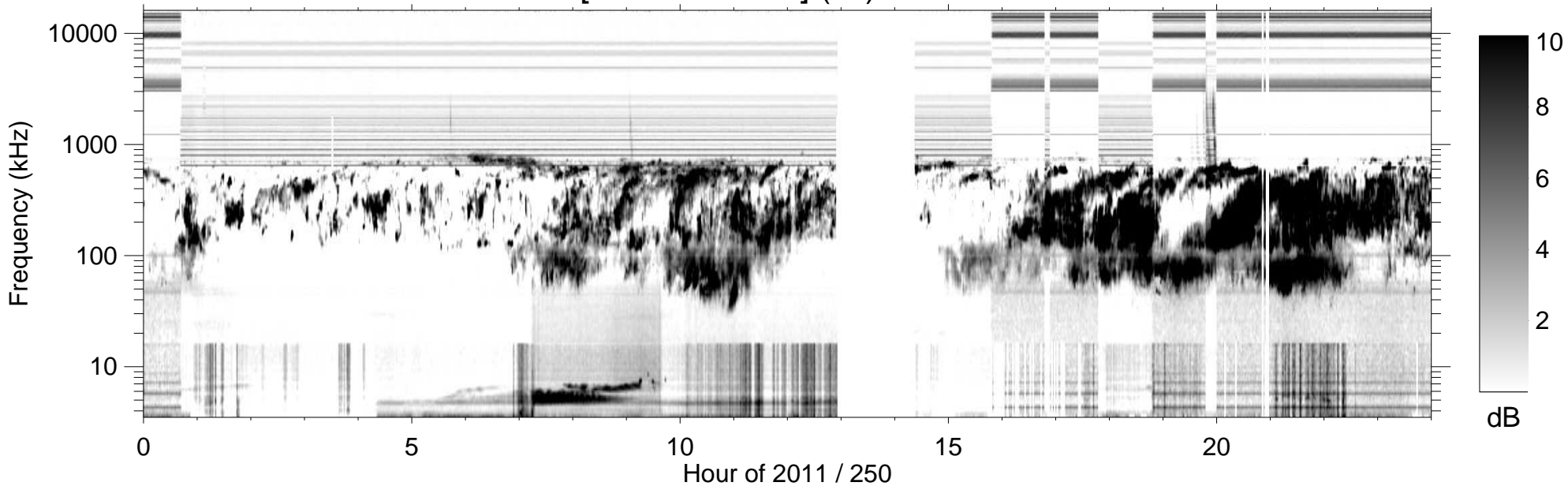
RPWS [ABCH1H2/Ex] (-B) 2011/09/07
