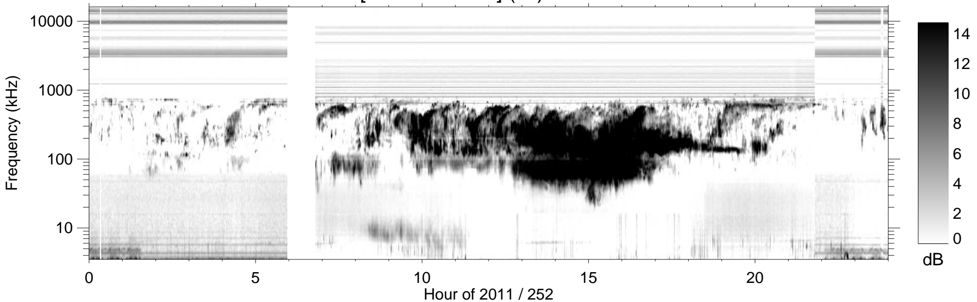
RPWS [ABCH1H2/Ex] (-B) 2011/09/09
