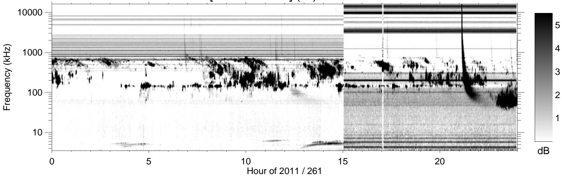
RPWS [ABCH1H2/Ex] (-B) 2011/09/18
