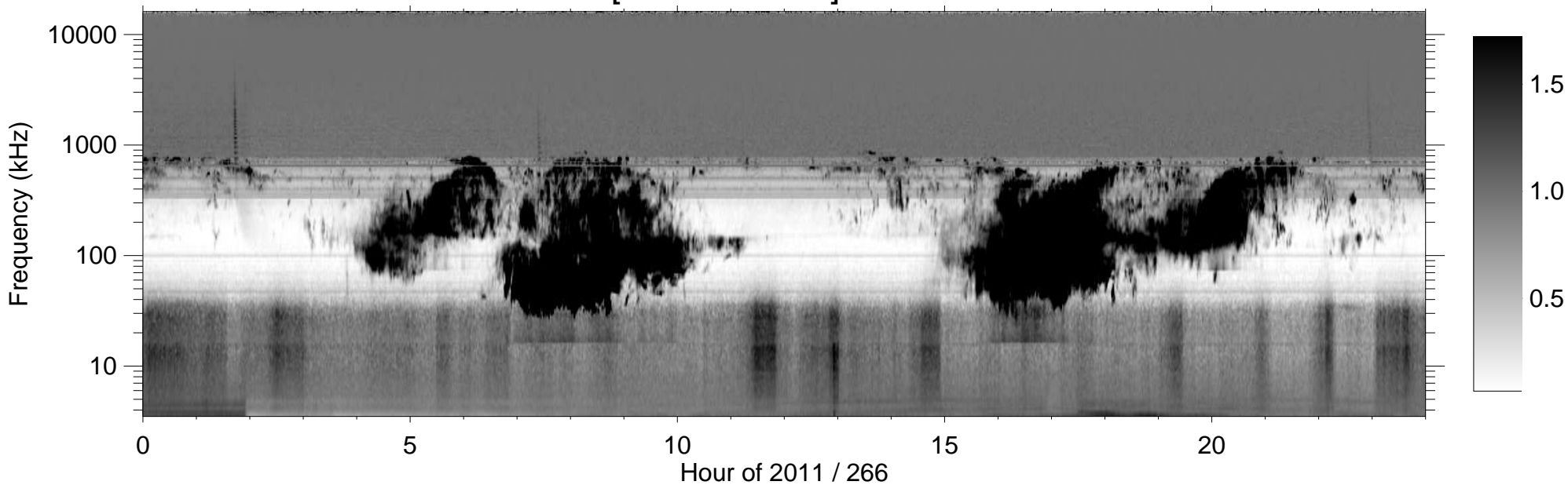
RPWS [ABCH1H2/Ex] (-B) 2011/09/23
