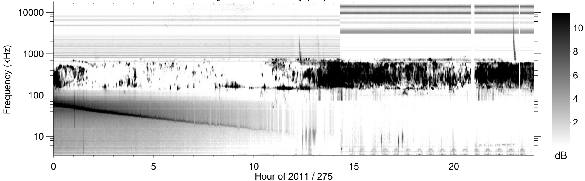
RPWS [ABCH1H2/Ex] (-B) 2011/10/02
