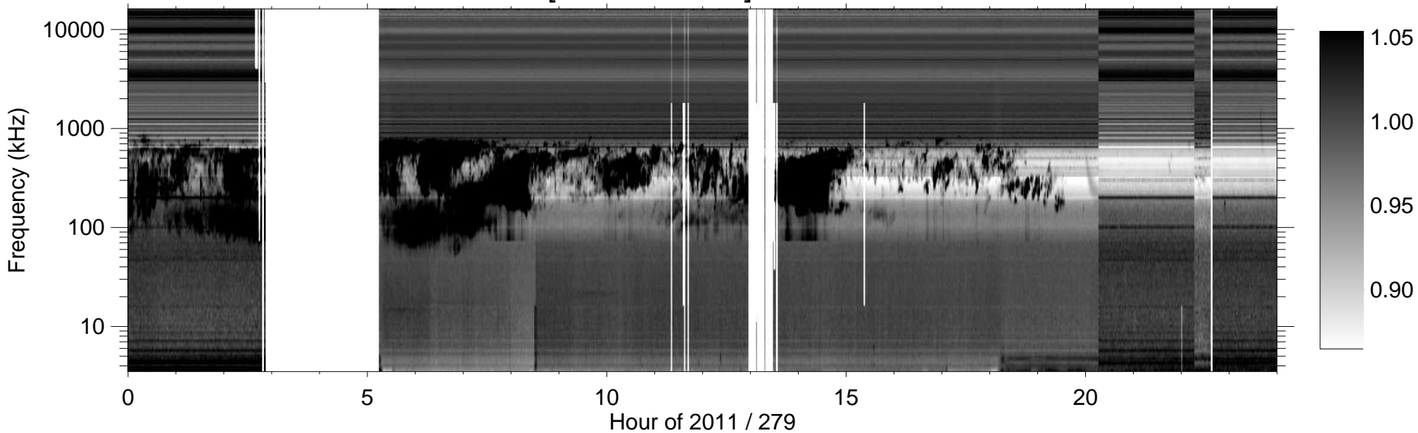
RPWS [ABCH1H2/Ex] (-B) 2011/10/06
