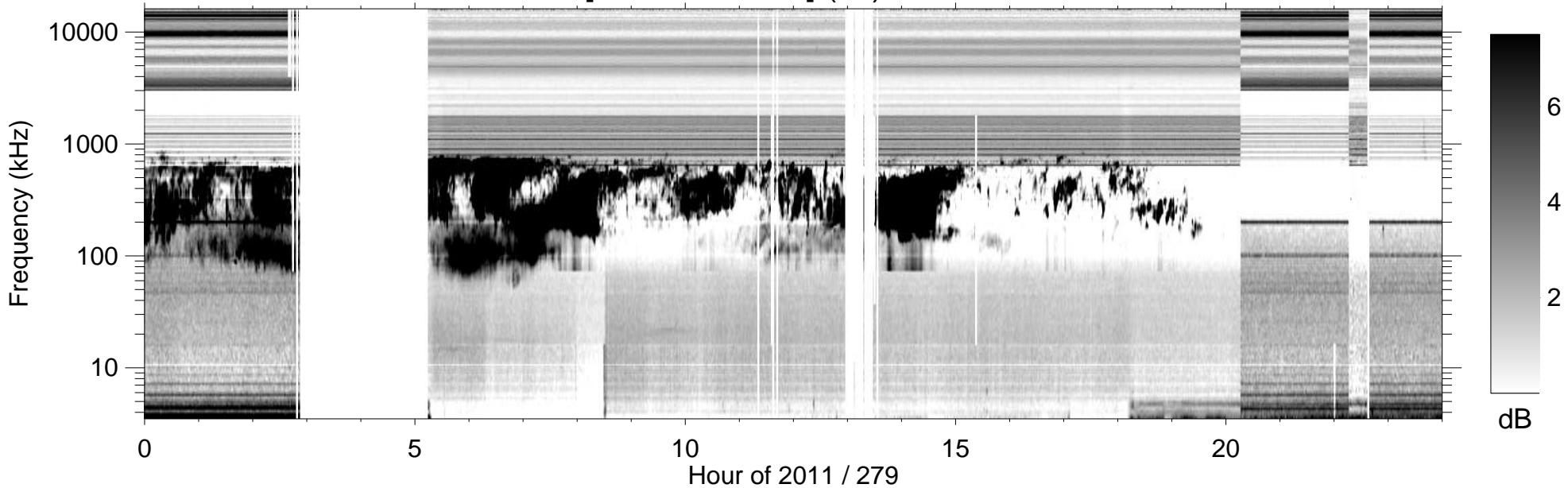
RPWS [ABCH1H2/Ex] (-B) 2011/10/06
