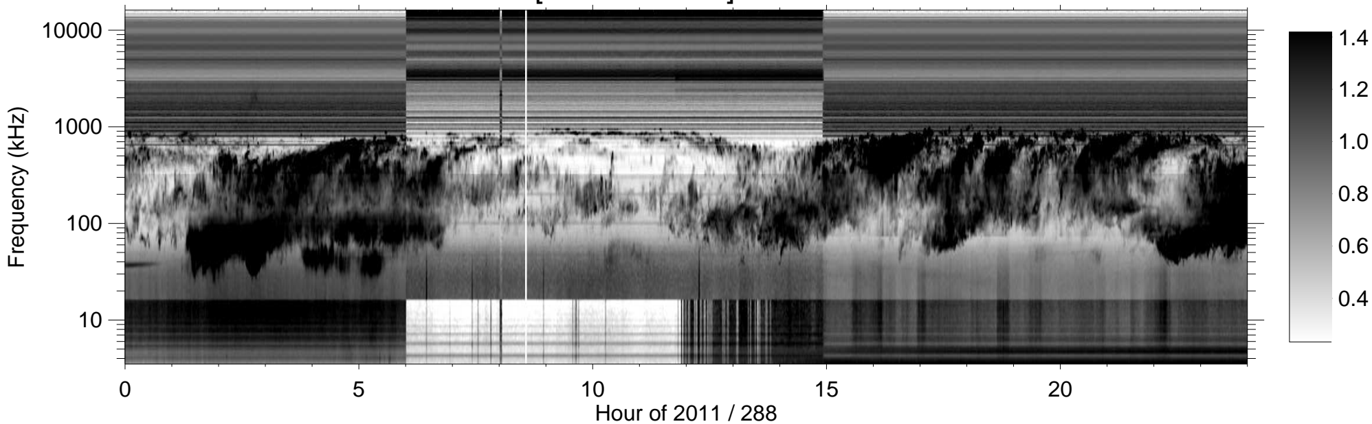
RPWS [ABCH1H2/Ex] (-B) 2011/10/15
