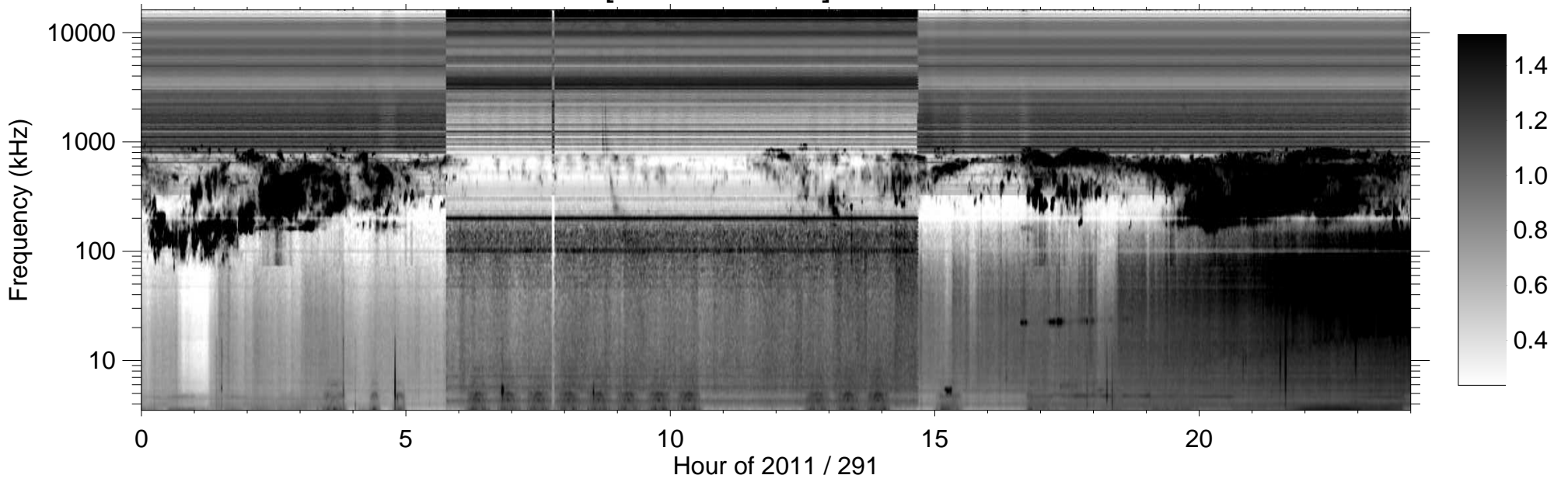
RPWS [ABCH1H2/Ex] (-B) 2011/10/18
