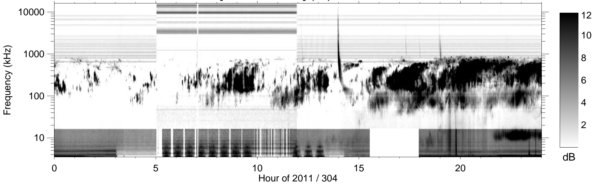
RPWS [ABCH1H2/Ex] (-B) 2011/10/31
