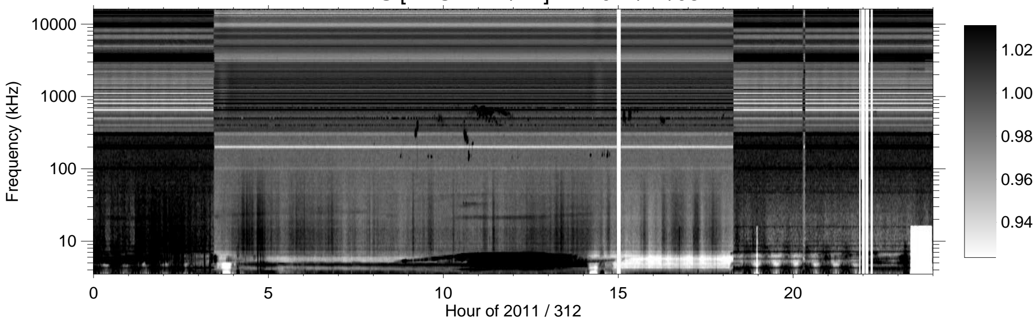
RPWS [ABCH1H2/Ex] (-B) 2011/11/08
