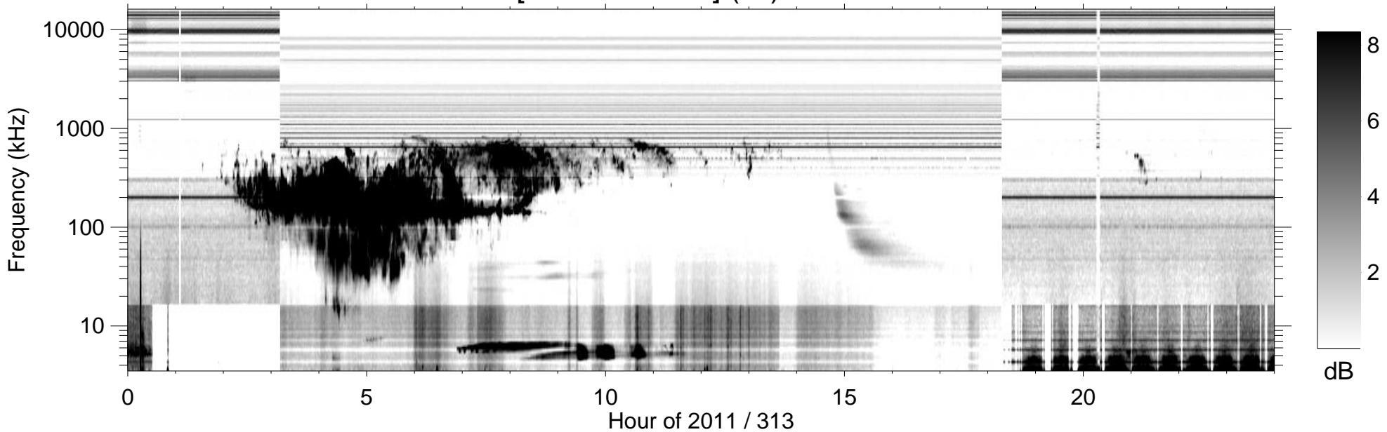
RPWS [ABCH1H2/Ex] (-B) 2011/11/09
