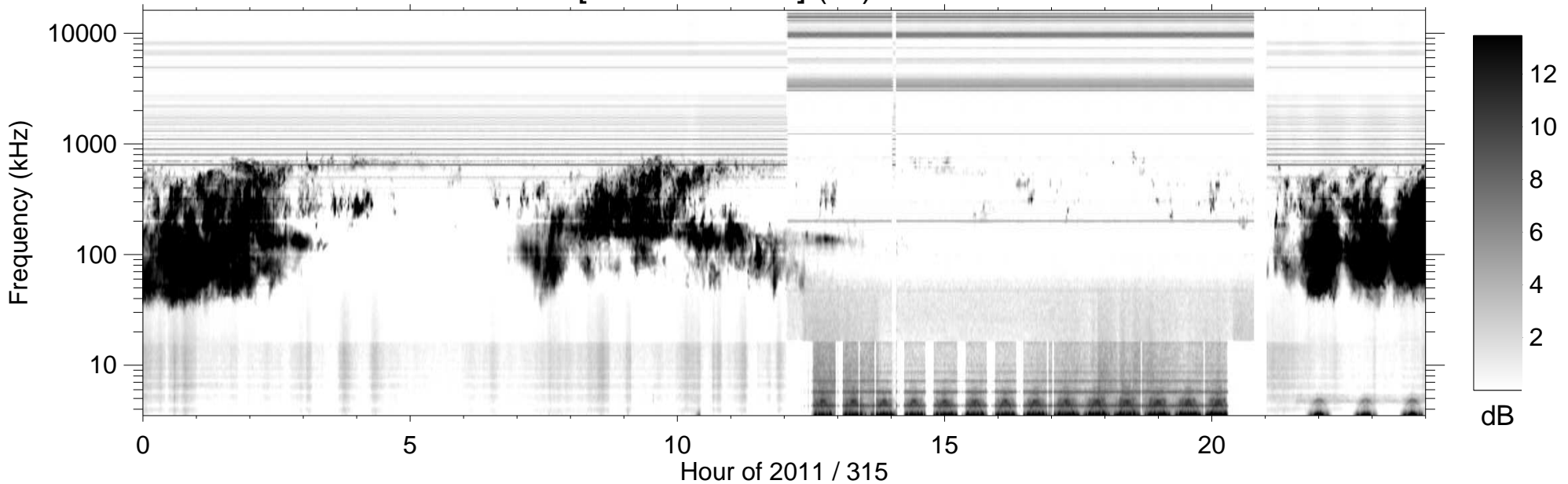
RPWS [ABCH1H2/Ex] (-B) 2011/11/11
