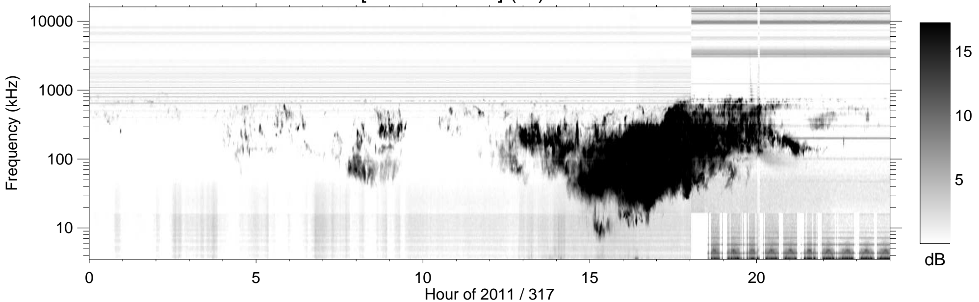
RPWS [ABCH1H2/Ex] (-B) 2011/11/13
