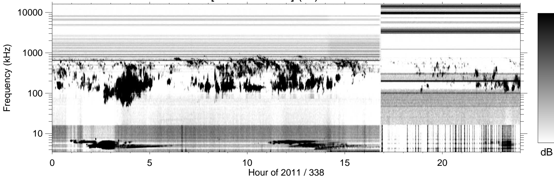
RPWS [ABCH1H2/Ex] (-B) 2011/12/04
