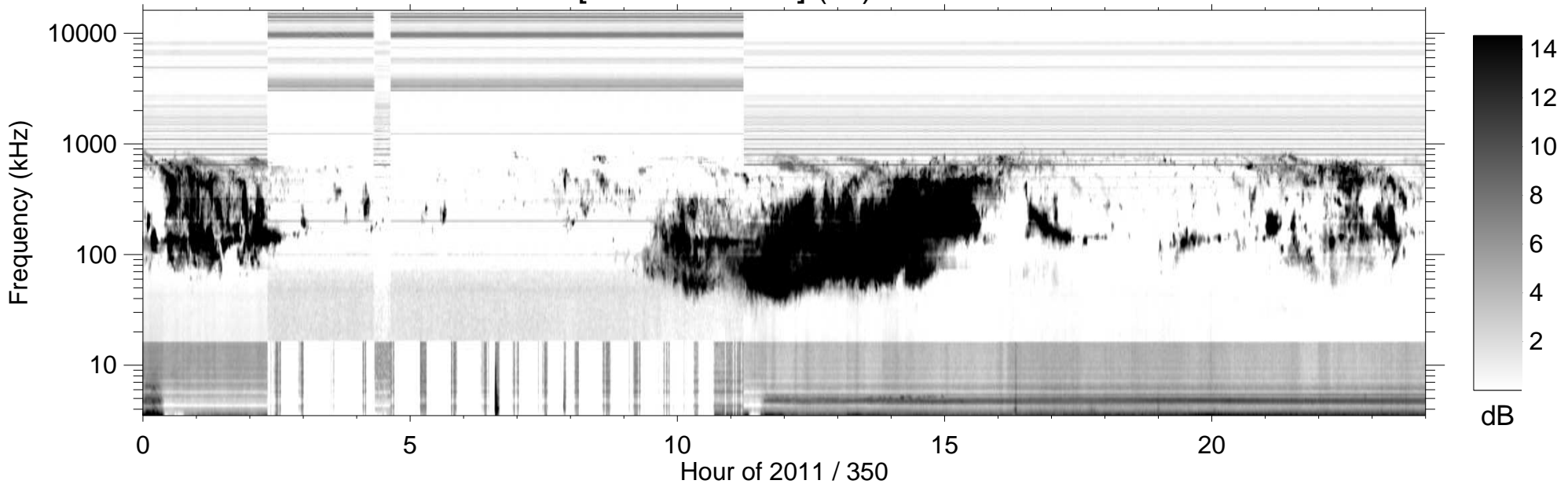
RPWS [ABCH1H2/Ex] (-B) 2011/12/16
