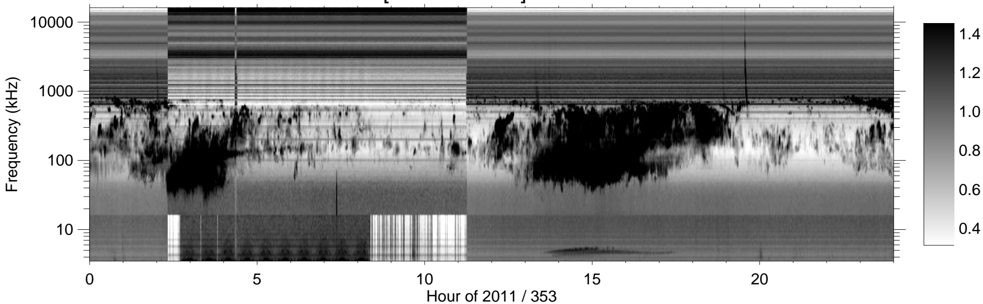
RPWS [ABCH1H2/Ex] (-B) 2011/12/19
