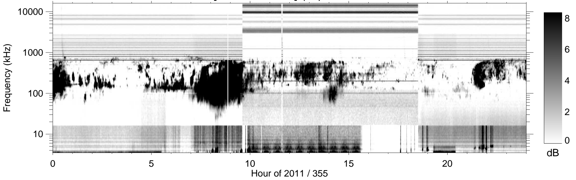
RPWS [ABCH1H2/Ex] (-B) 2011/12/21
