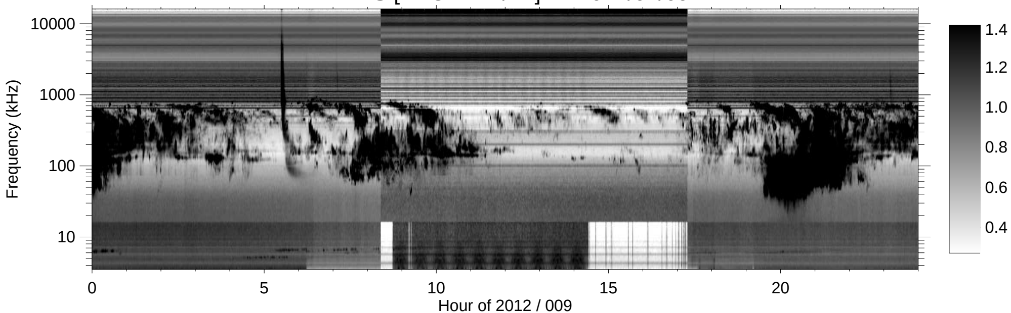
RPWS [ABCH1H2/Ex] (-B) 2012/01/09
