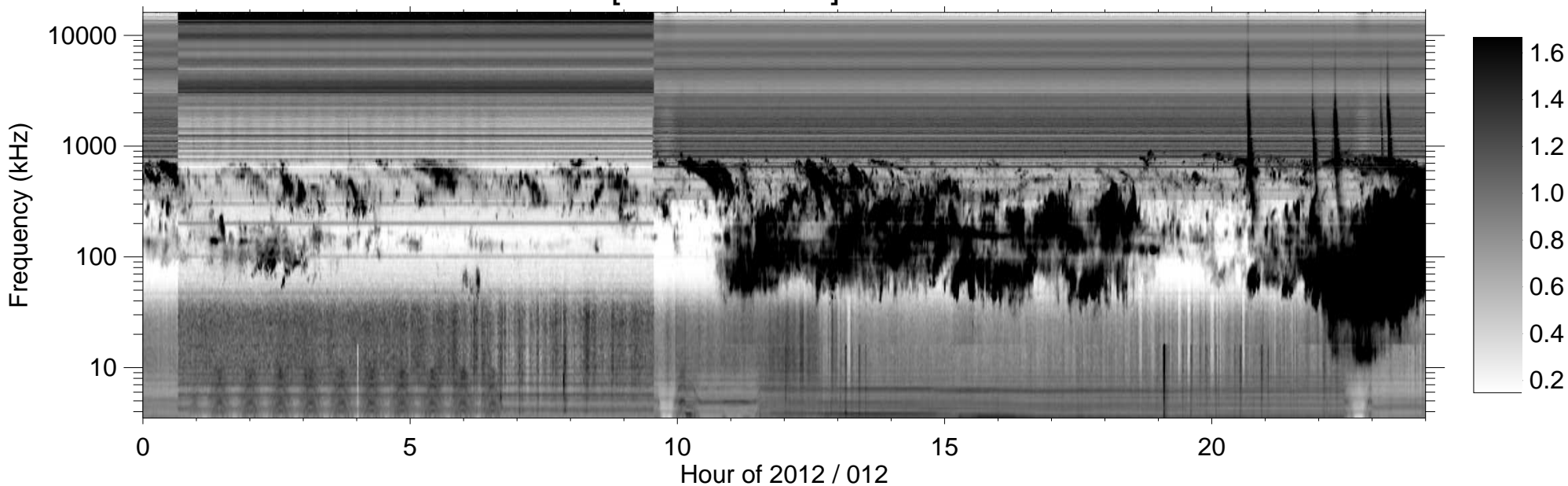
RPWS [ABCH1H2/Ex] (-B) 2012/01/12
