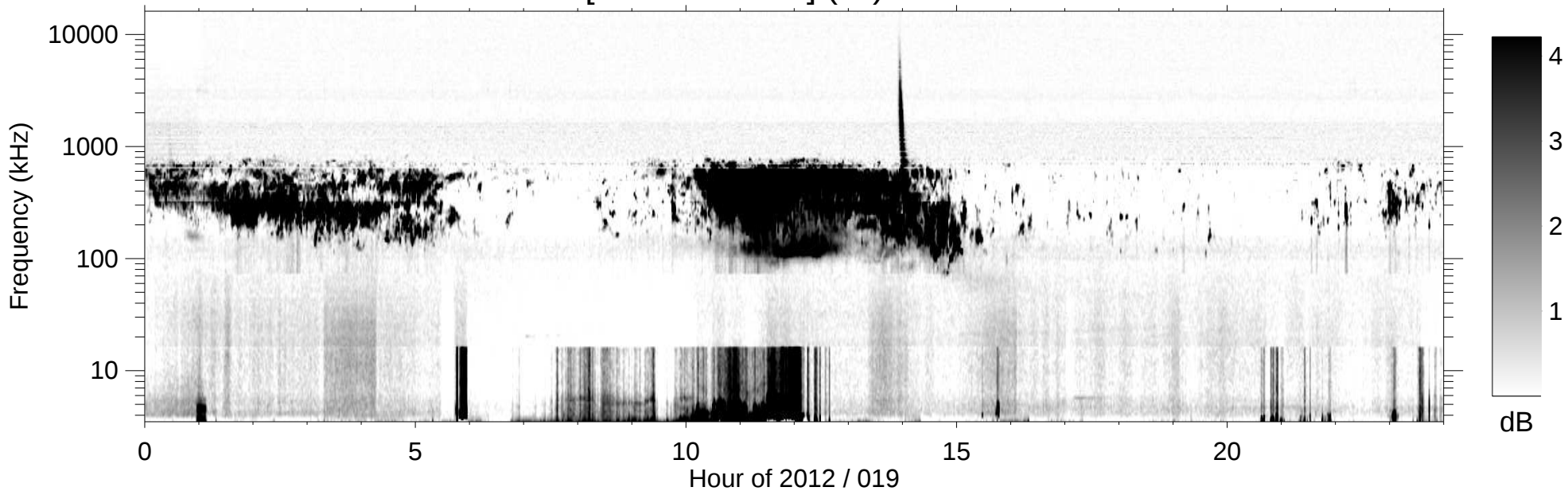
RPWS [ABCH1H2/Ex] (-B) 2012/01/19
