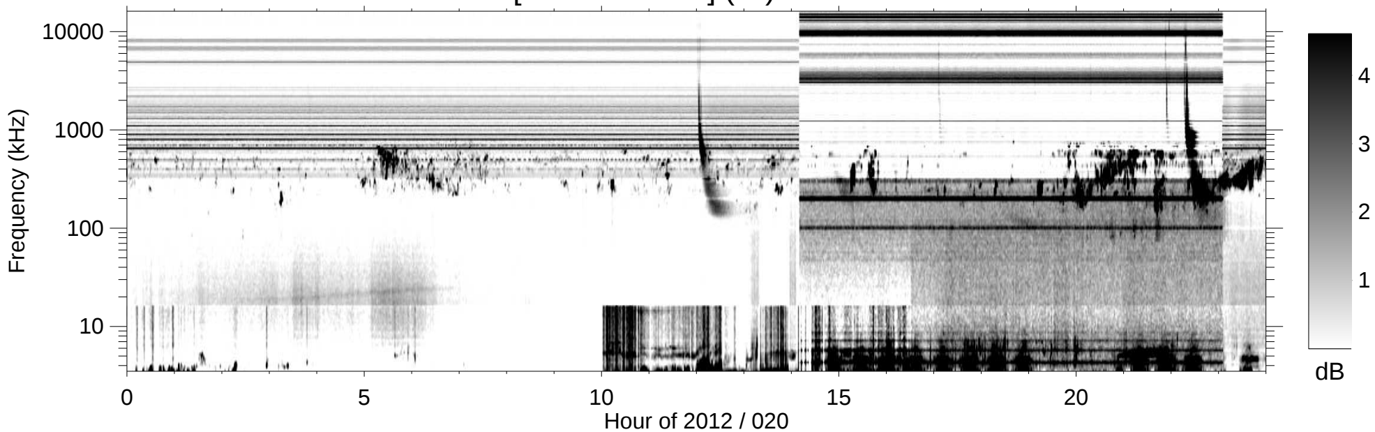
RPWS [ABCH1H2/Ex] (-B) 2012/01/20
