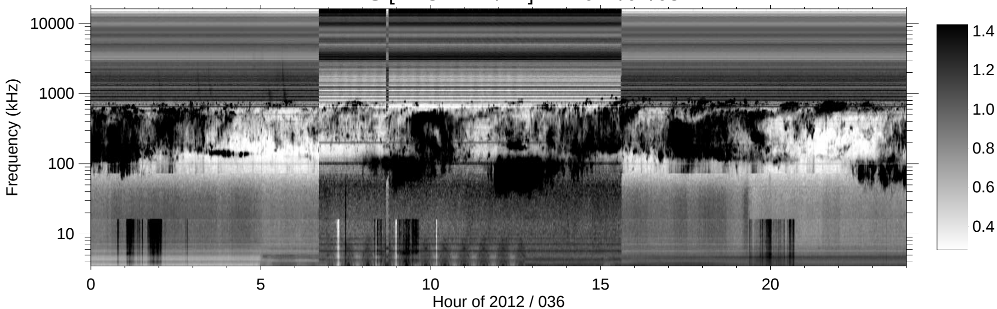
RPWS [ABCH1H2/Ex] (-B) 2012/02/05
