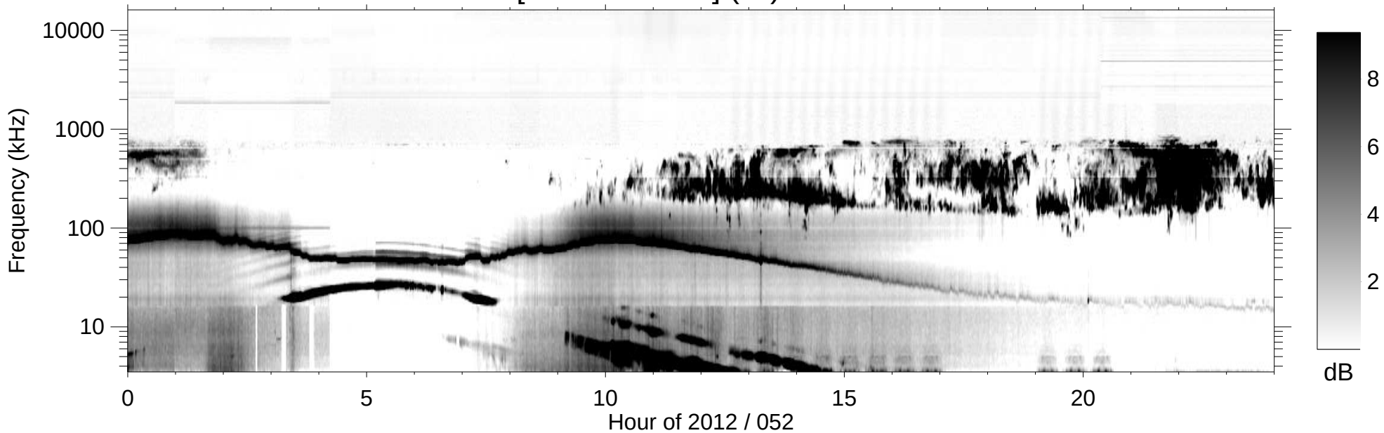
RPWS [ABCH1H2/Ex] (-B) 2012/02/21
