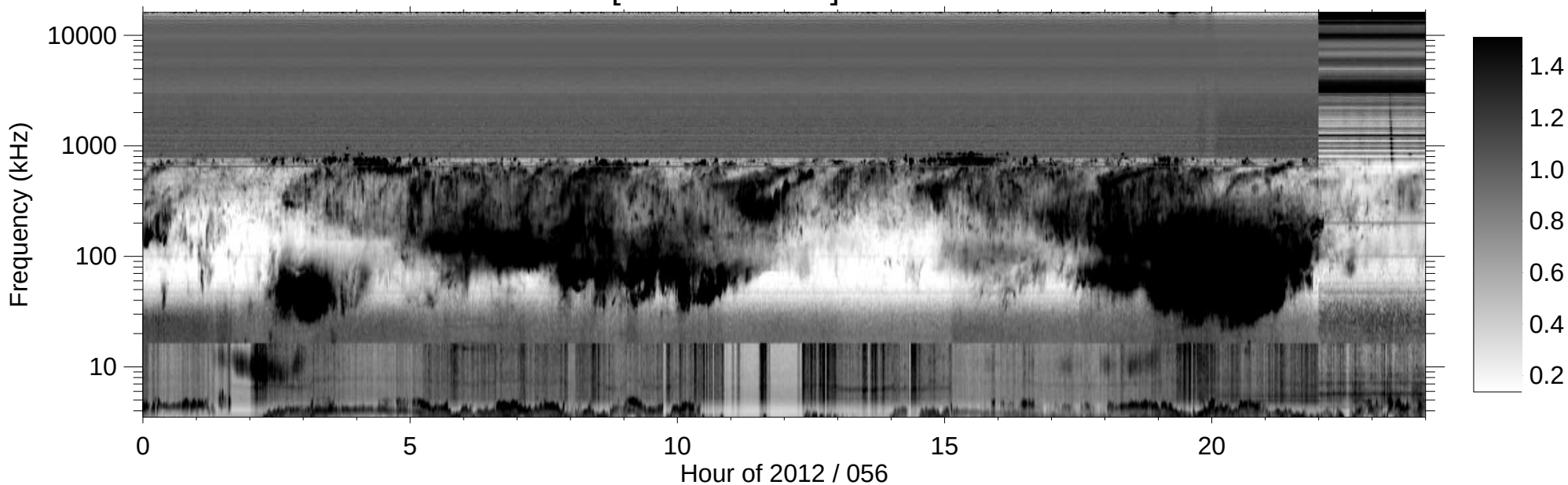
RPWS [ABCH1H2/Ex] (-B) 2012/02/25
