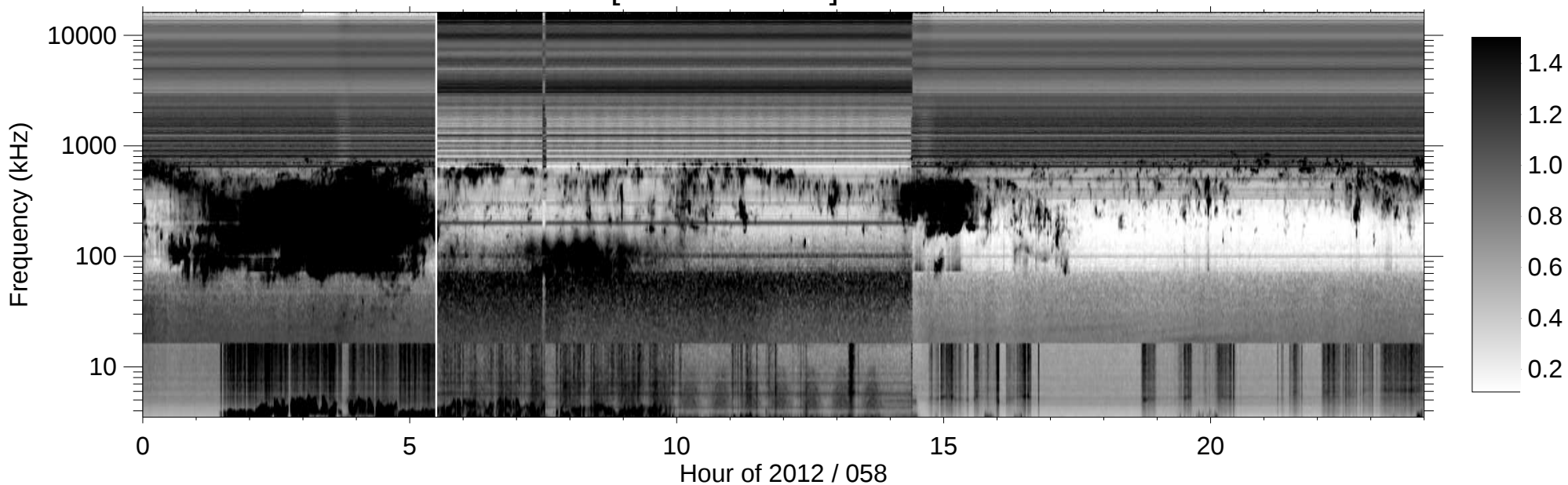
RPWS [ABCH1H2/Ex] (-B) 2012/02/27
