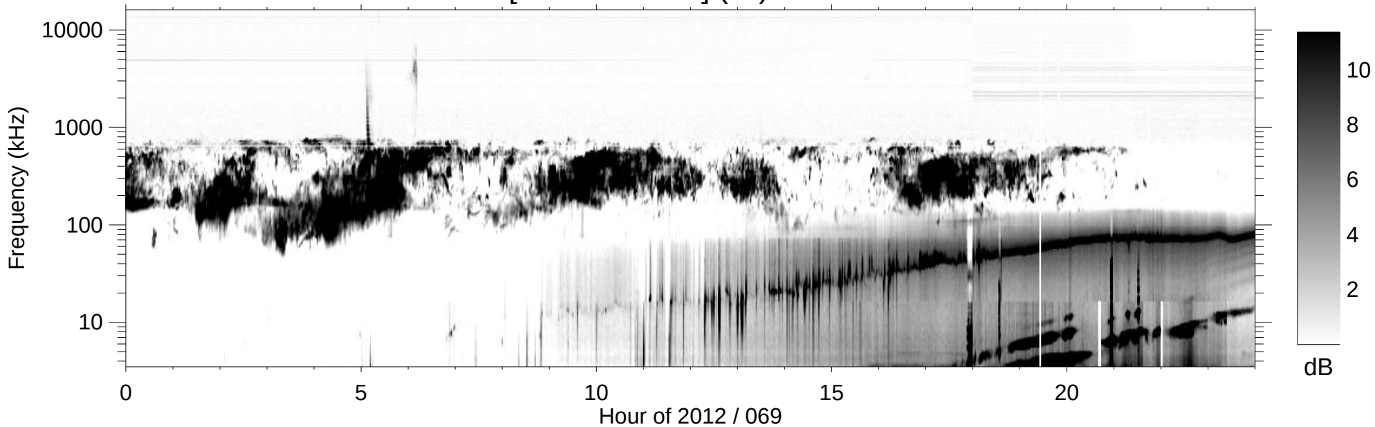
RPWS [ABCH1H2/Ex] (-B) 2012/03/09
