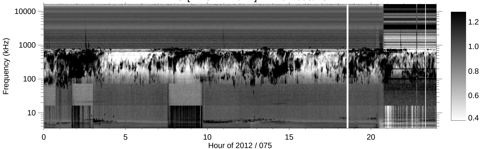
RPWS [ABCH1H2/Ex] (-B) 2012/03/15
