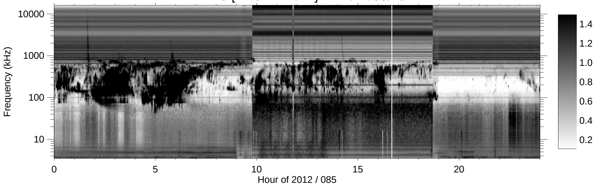
RPWS [ABCH1H2/Ex] (-B) 2012/03/25
