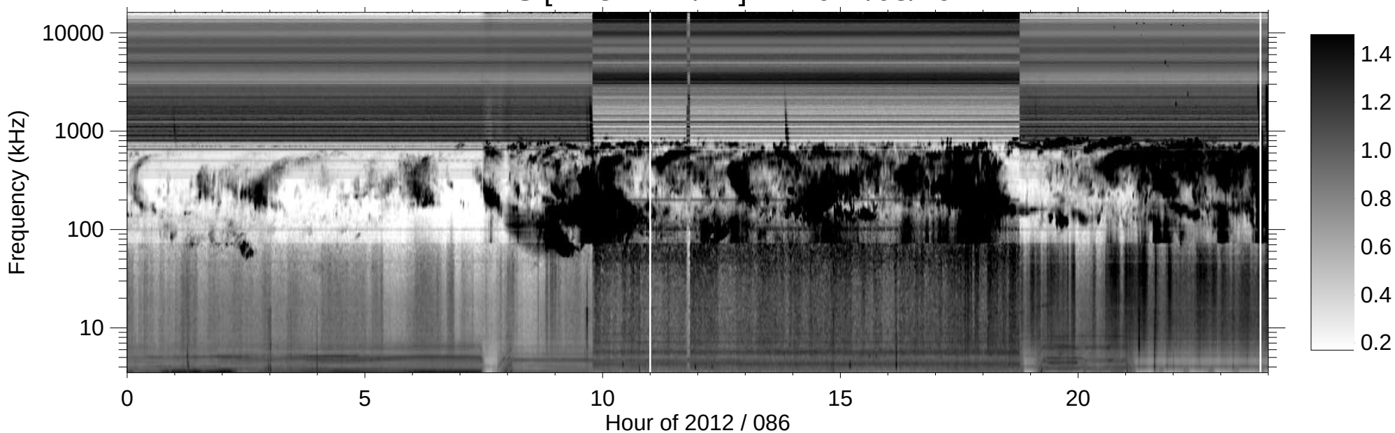
RPWS [ABCH1H2/Ex] (-B) 2012/03/26
