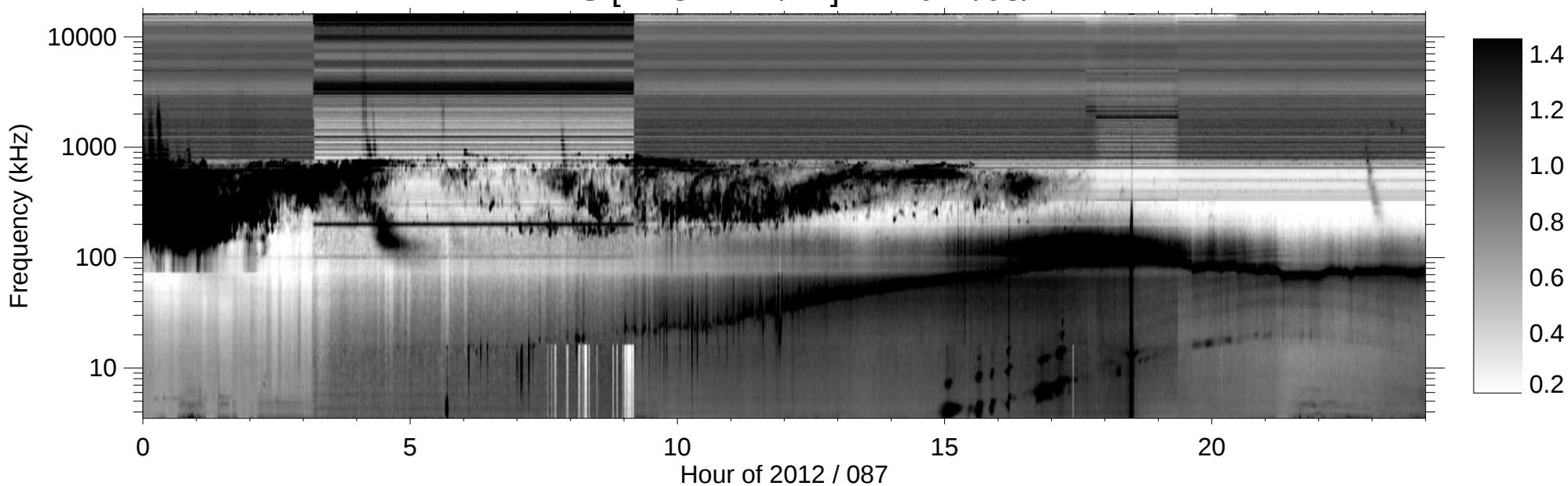
RPWS [ABCH1H2/Ex] (-B) 2012/03/27
