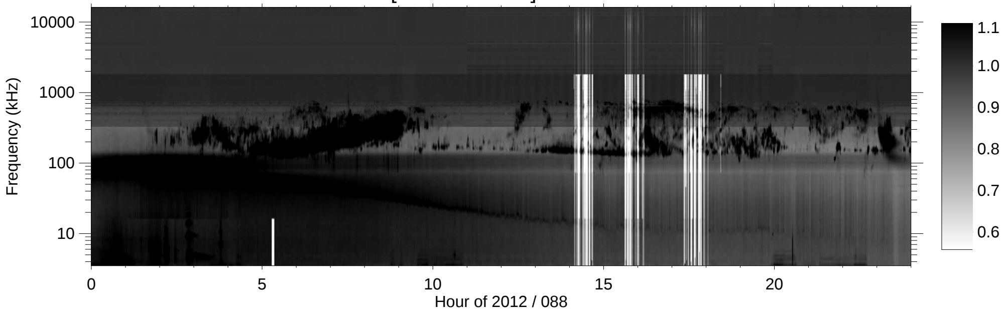
RPWS [ABCH1H2/Ex] (-B) 2012/03/28
