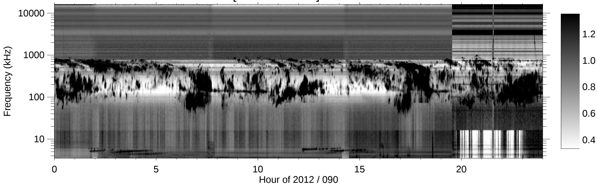
RPWS [ABCH1H2/Ex] (-B) 2012/03/30
