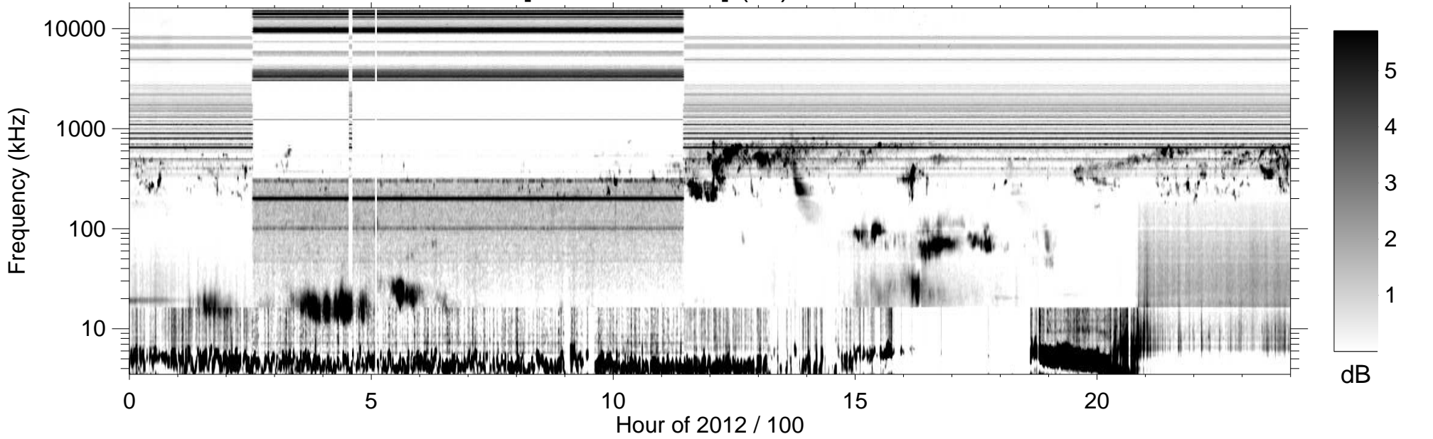
RPWS [ABCH1H2/Ex] (-B) 2012/04/09
