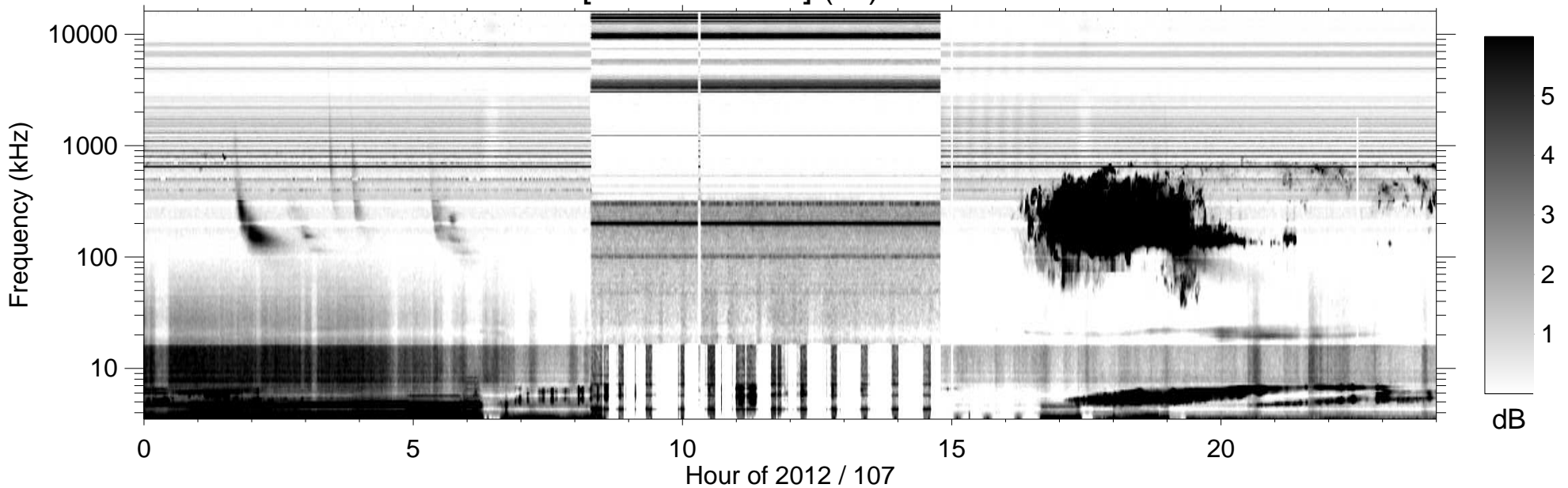
RPWS [ABCH1H2/Ex] (-B) 2012/04/16
