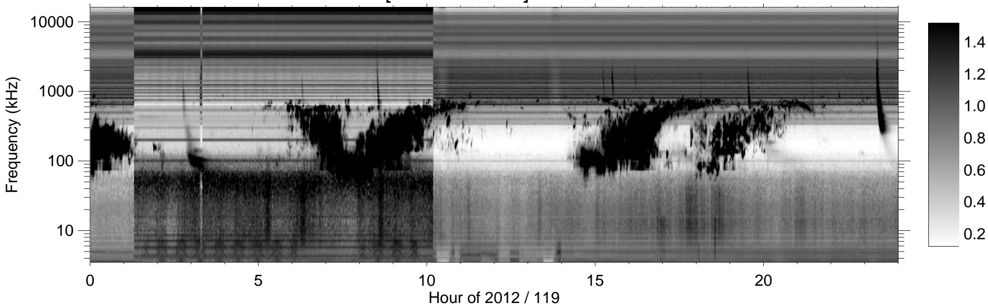
RPWS [ABCH1H2/Ex] (-B) 2012/04/28
