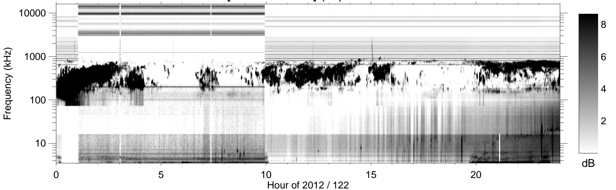
RPWS [ABCH1H2/Ex] (-B) 2012/05/01
