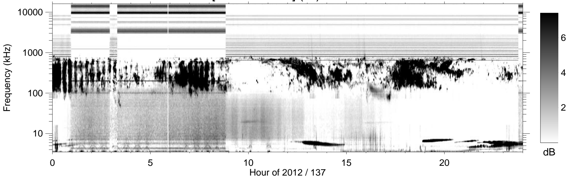
RPWS [ABCH1H2/Ex] (-B) 2012/05/16
