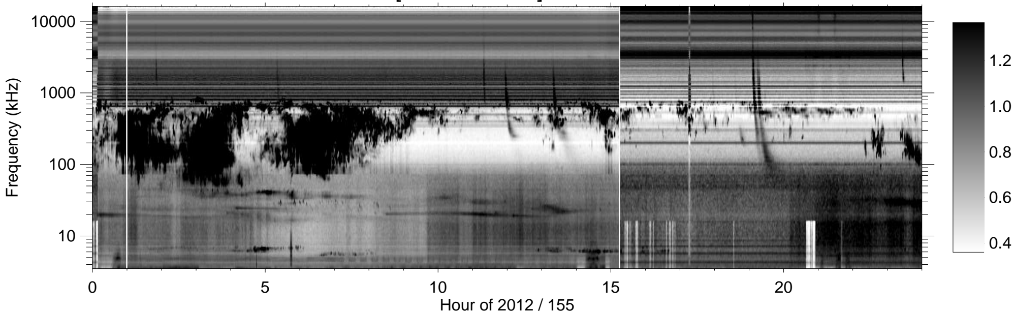
RPWS [ABCH1H2/Ex] (-B) 2012/06/03
