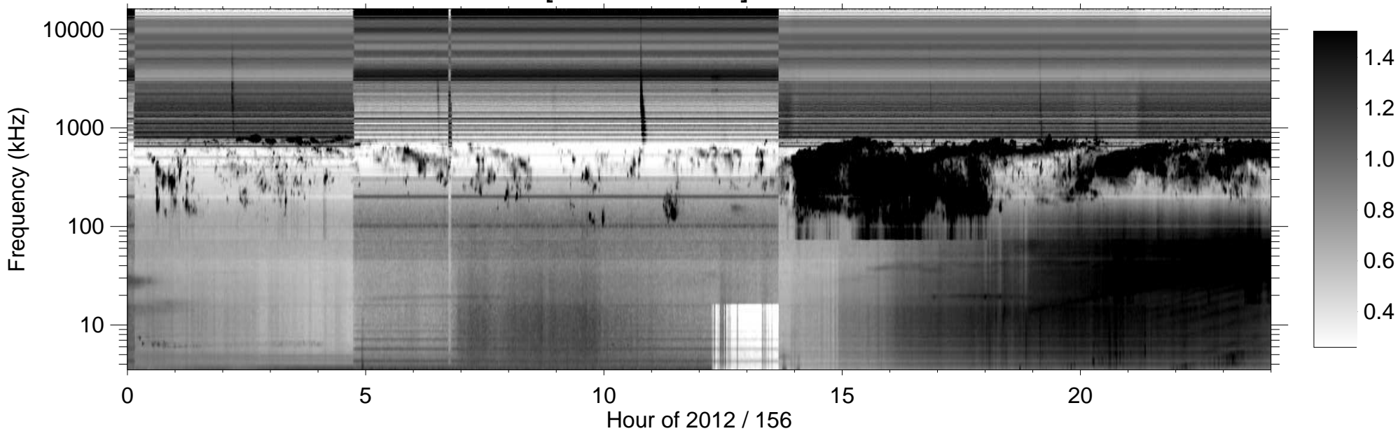
RPWS [ABCH1H2/Ex] (-B) 2012/06/04
