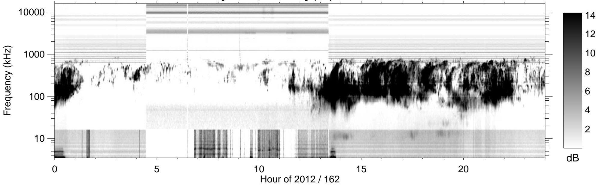
RPWS [ABCH1H2/Ex] (-B) 2012/06/10
