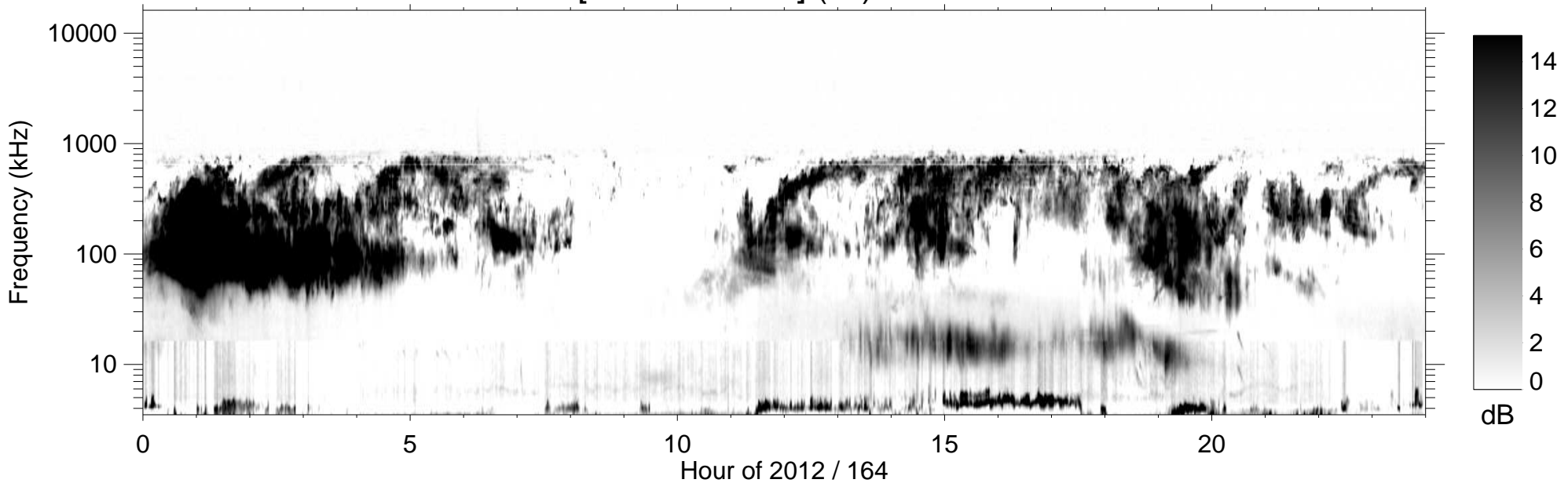
RPWS [ABCH1H2/Ex] (-B) 2012/06/12
