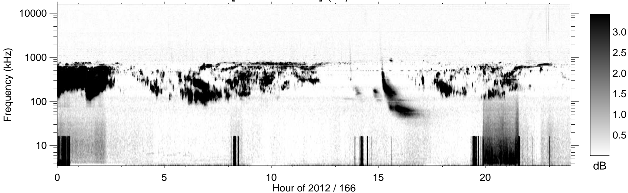
RPWS [ABCH1H2/Ex] (-B) 2012/06/14
