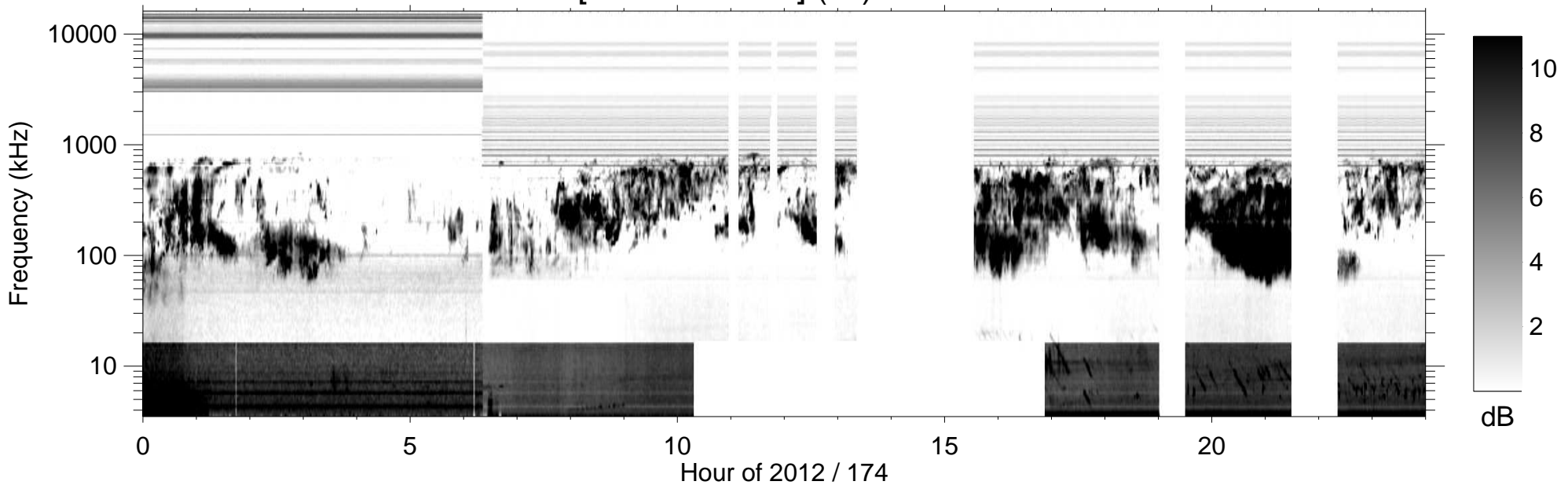
RPWS [ABCH1H2/Ex] (-B) 2012/06/22
