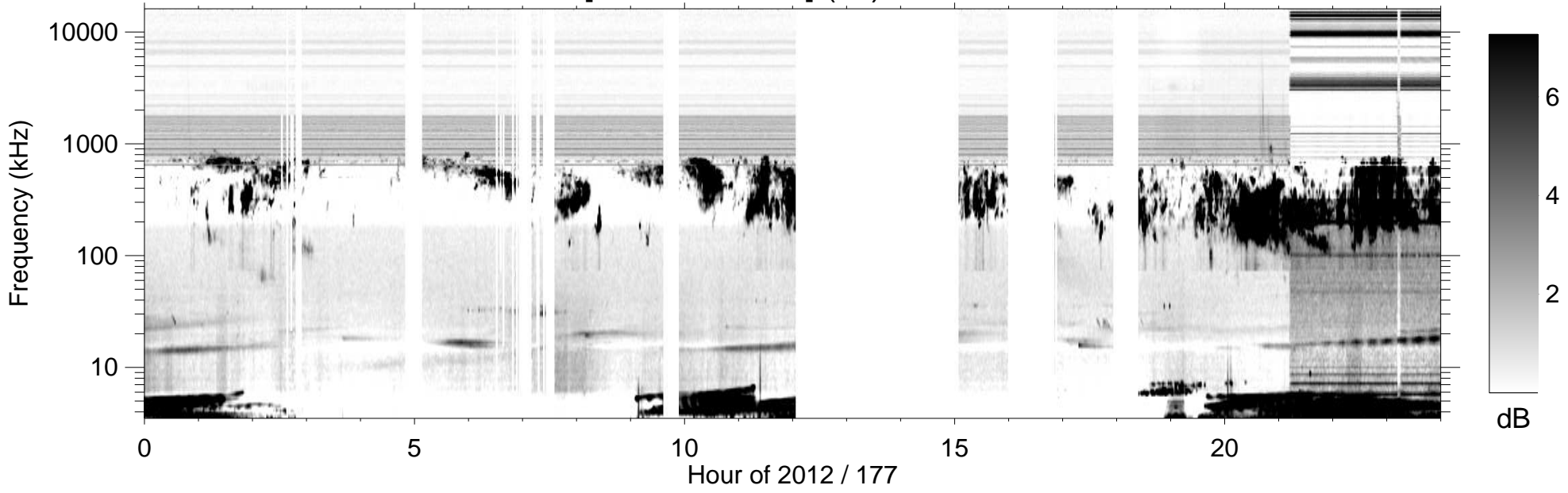
RPWS [ABCH1H2/Ex] (-B) 2012/06/25
