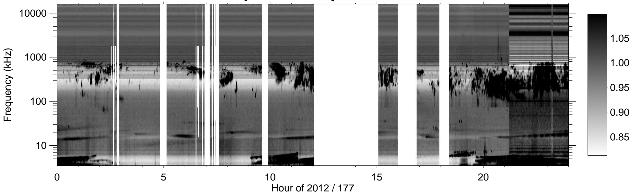
RPWS [ABCH1H2/Ex] (-B) 2012/06/25
