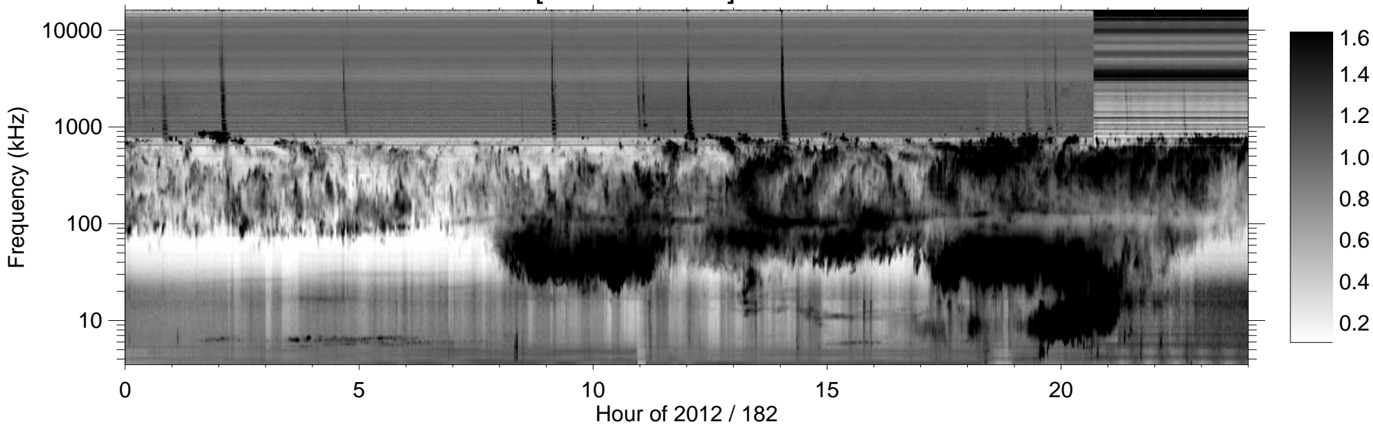
RPWS [ABCH1H2/Ex] (-B) 2012/06/30
