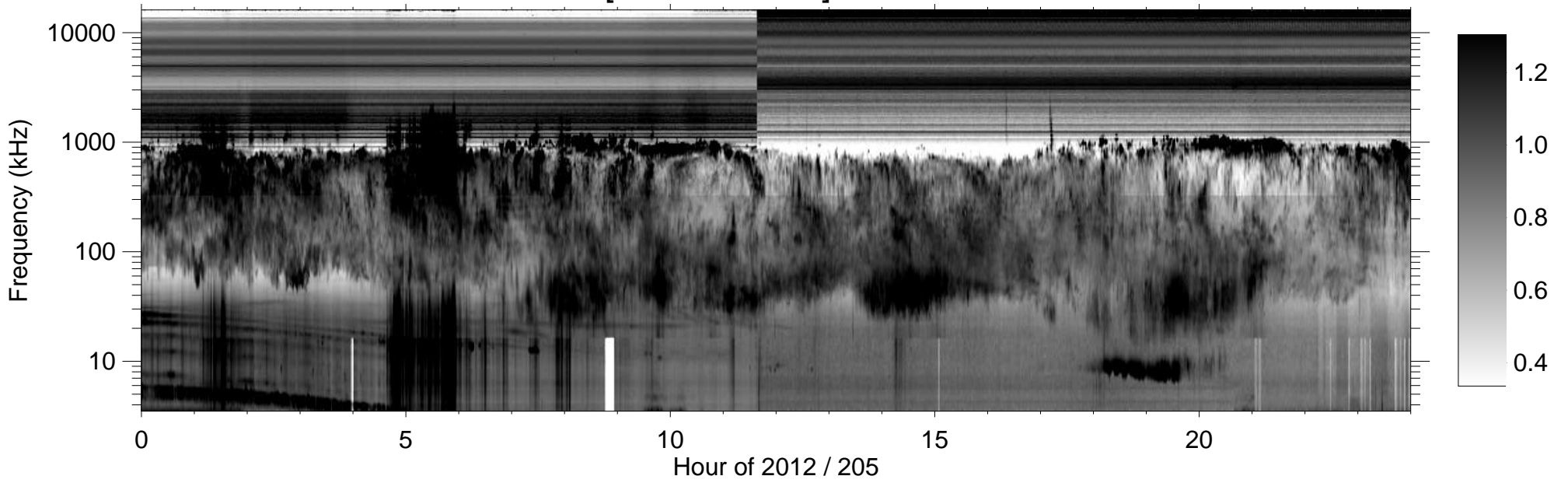
RPWS [ABCH1H2/Ex] (-B) 2012/07/23
