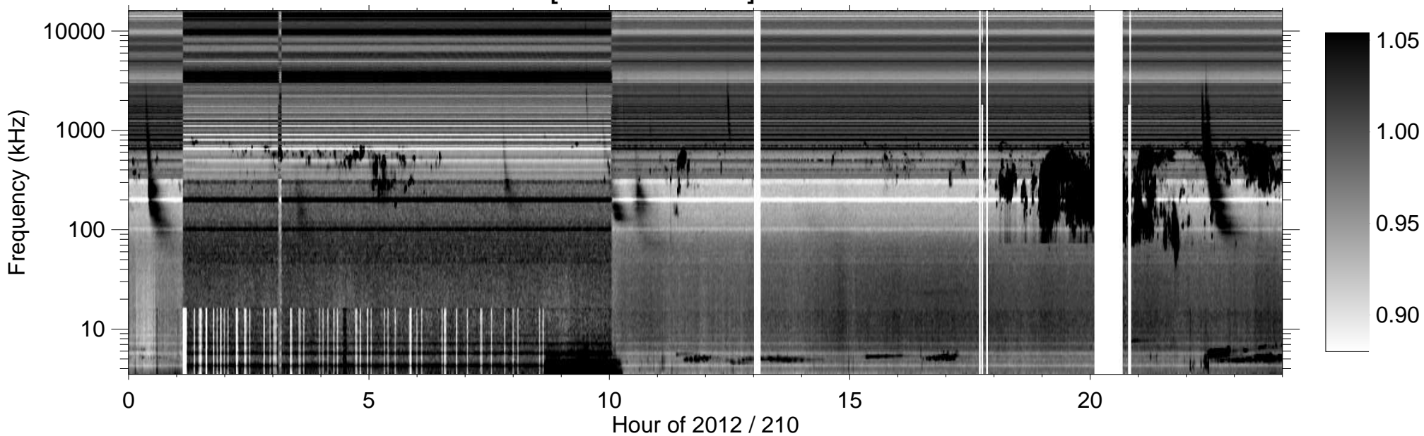
RPWS [ABCH1H2/Ex] (-B) 2012/07/28
