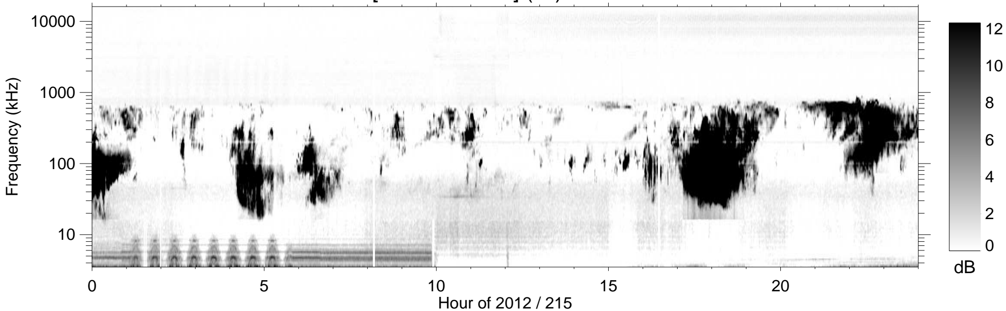
RPWS [ABCH1H2/Ex] (-B) 2012/08/02
