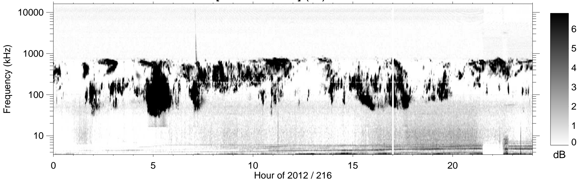
RPWS [ABCH1H2/Ex] (-B) 2012/08/03
